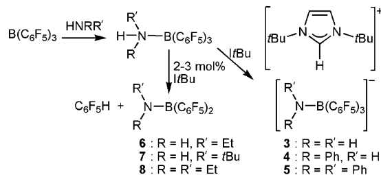
Scheme 3. N–H bond cleavage of amines with IrBu/B(C 6 F 5 ) 3 .
